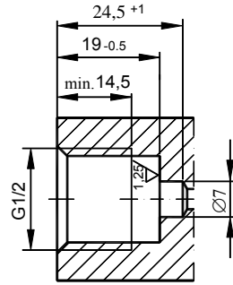
Fig.9b. Socket for G1/2-type connector.
