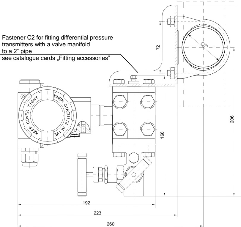
Fig. 14. Example: how to install the APR-2000ALW transmitter with a valve manifold to a 2" pipe.
