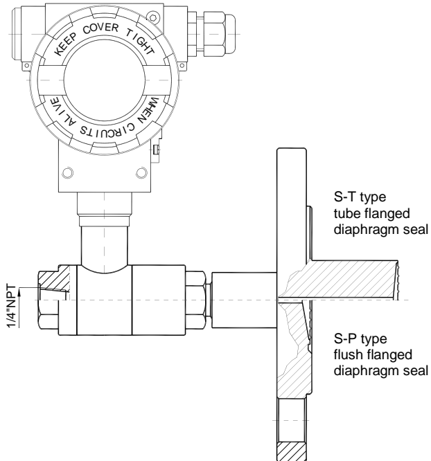
Fig. 11. APR-2000ALW differential pressure transmitter with a single direct diaphragm seal (example).
