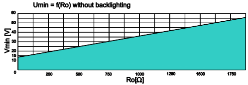
Safe working area for normal transmitter (grid) upper colour area.
